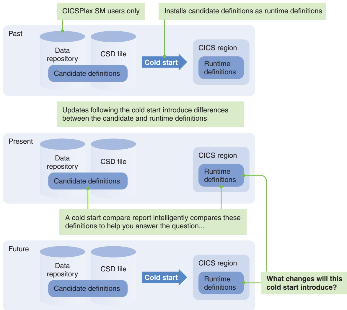
1 Figure 112. Deployment analysis reports: what will be the effect of cold starting a CICS region?
