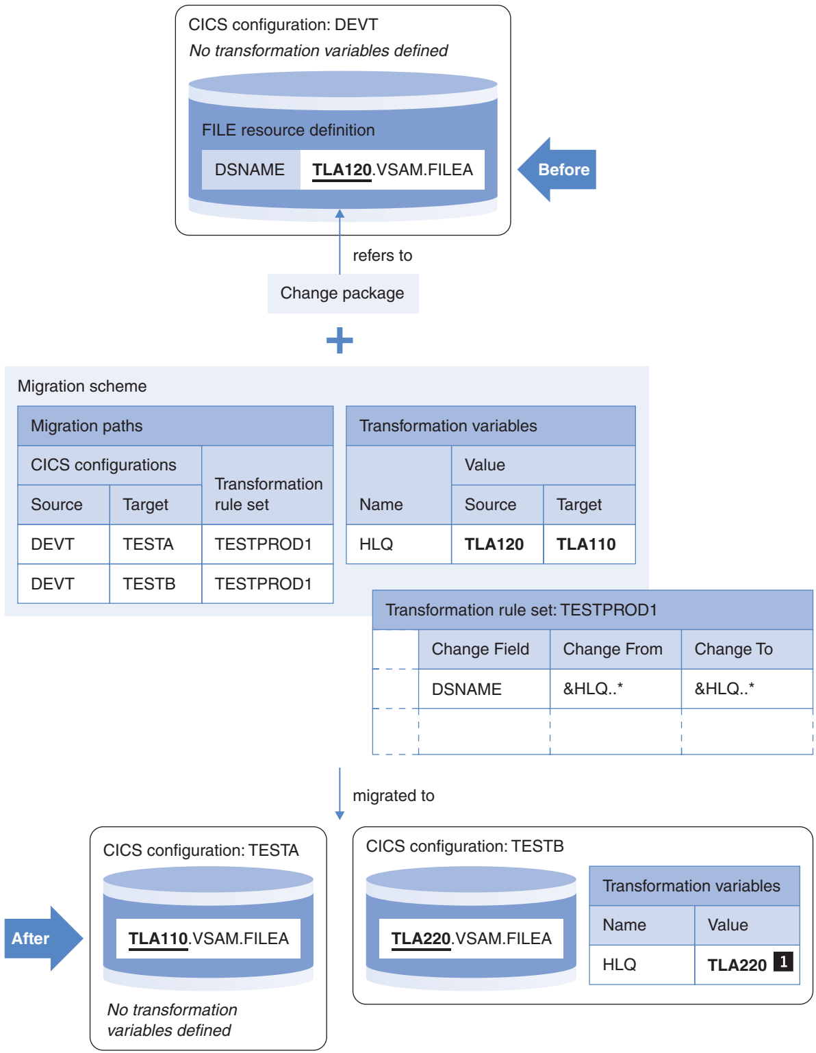
Figure 21. Example: using transformation variables
