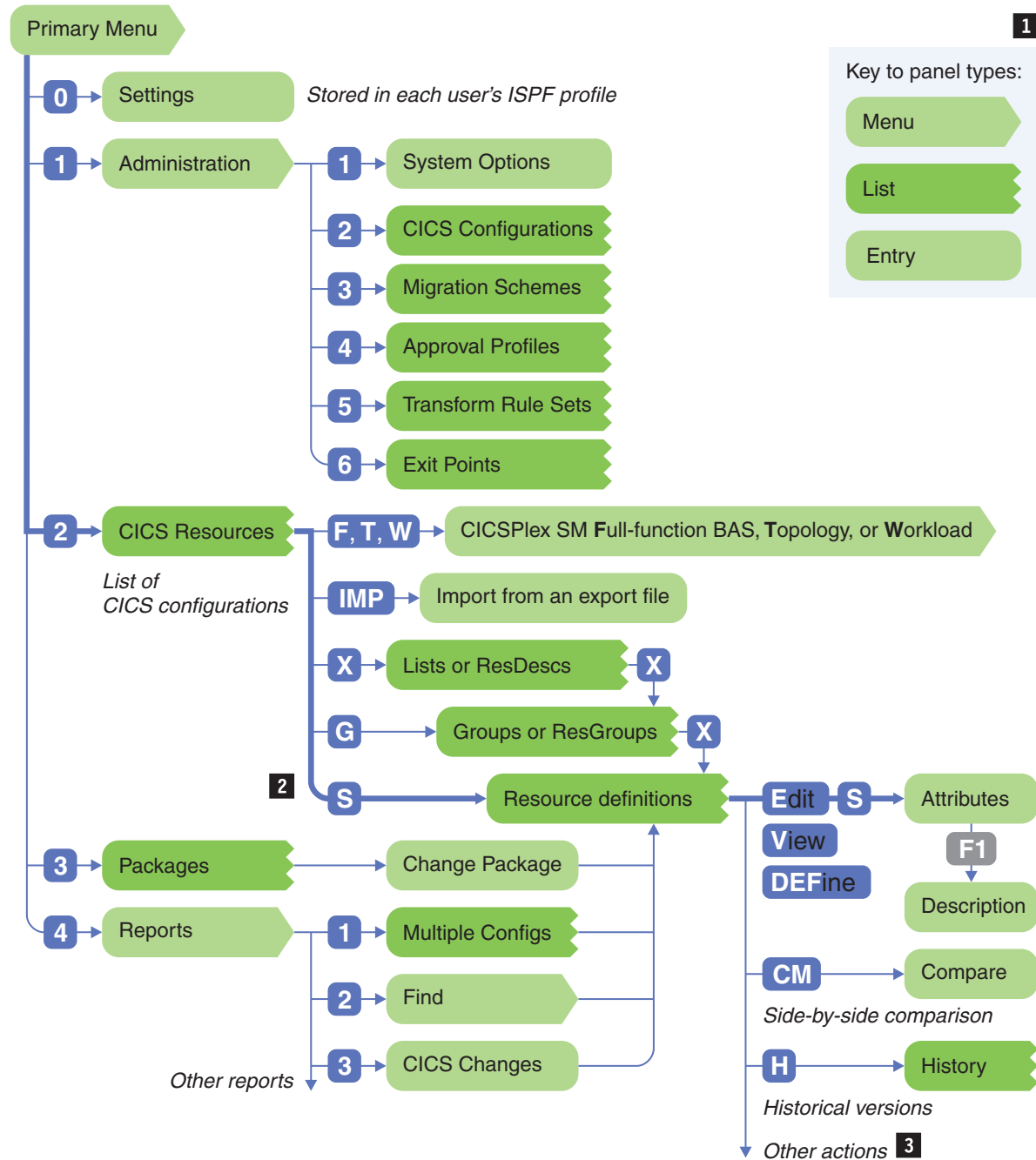
Figure 76. ISPF dialog panel hierarchy
