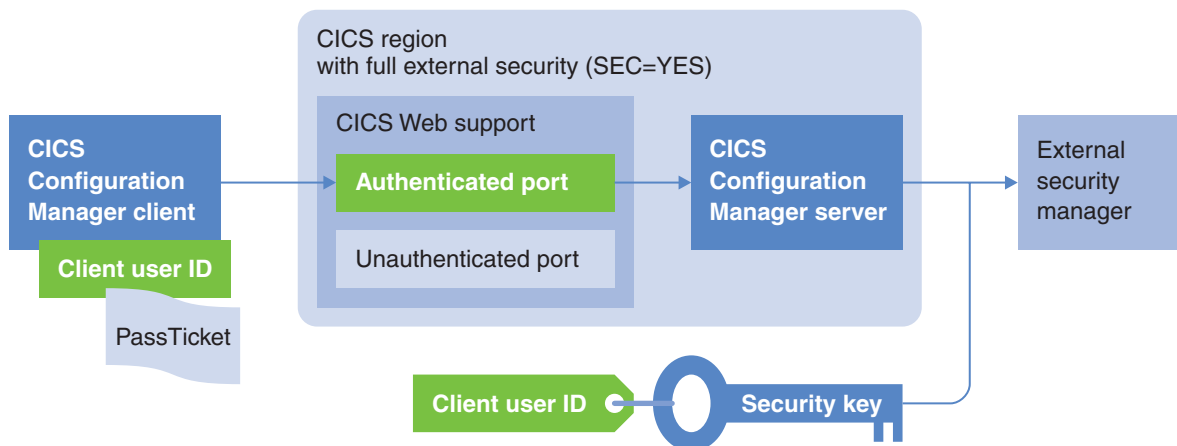
Figure 50. Connecting via an authenticated port: access is authorized by the client user ID
