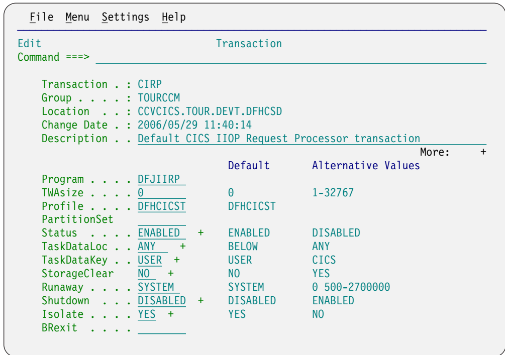
Figure 58. Guided tour: Viewing or editing the attributes of a resource definition
