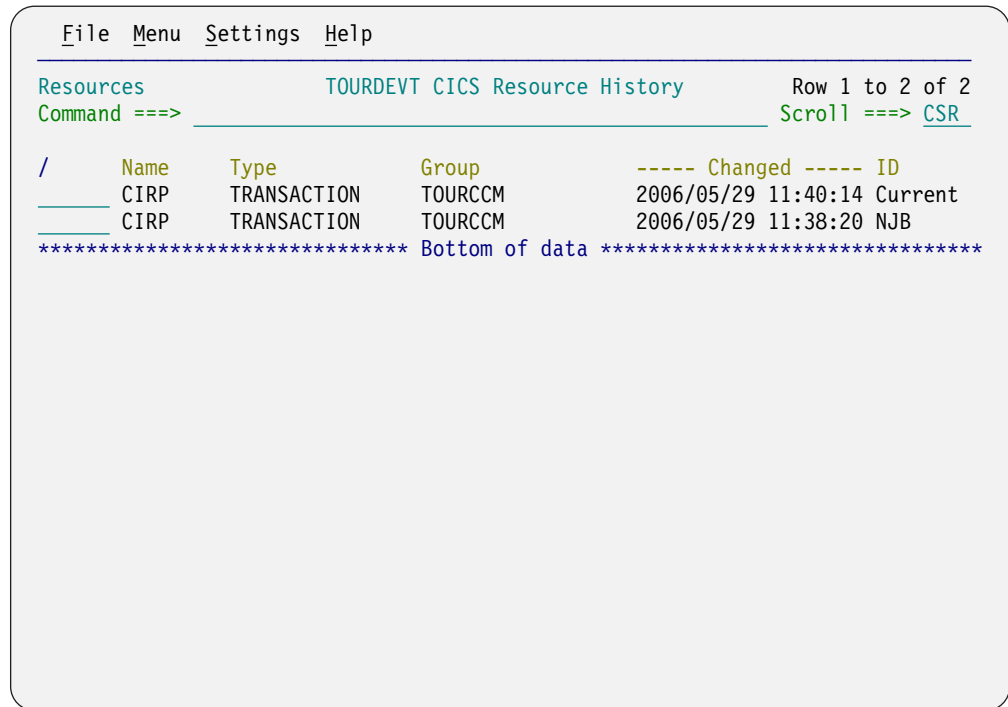
Figure 63. Guided tour: Displaying a list of historical versions of a resource definition
