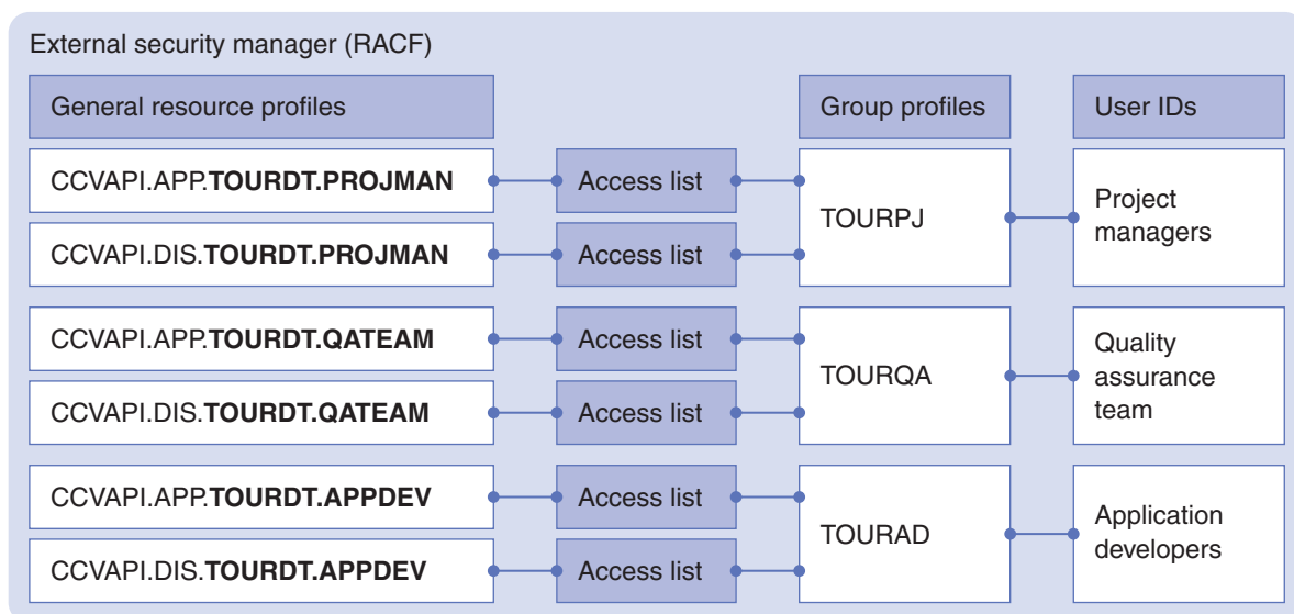
Figure 74. Guided tour: Normal migration from development to test requires approval by three approver roles
