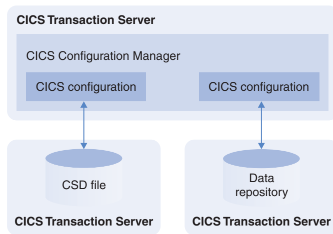
Figure 123. Example usage involving several instances of CICS Transaction Server
