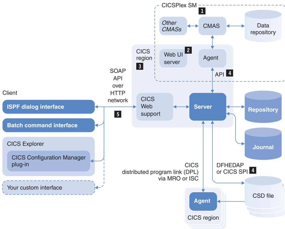
Figure 8. CICS Configuration Manager components
