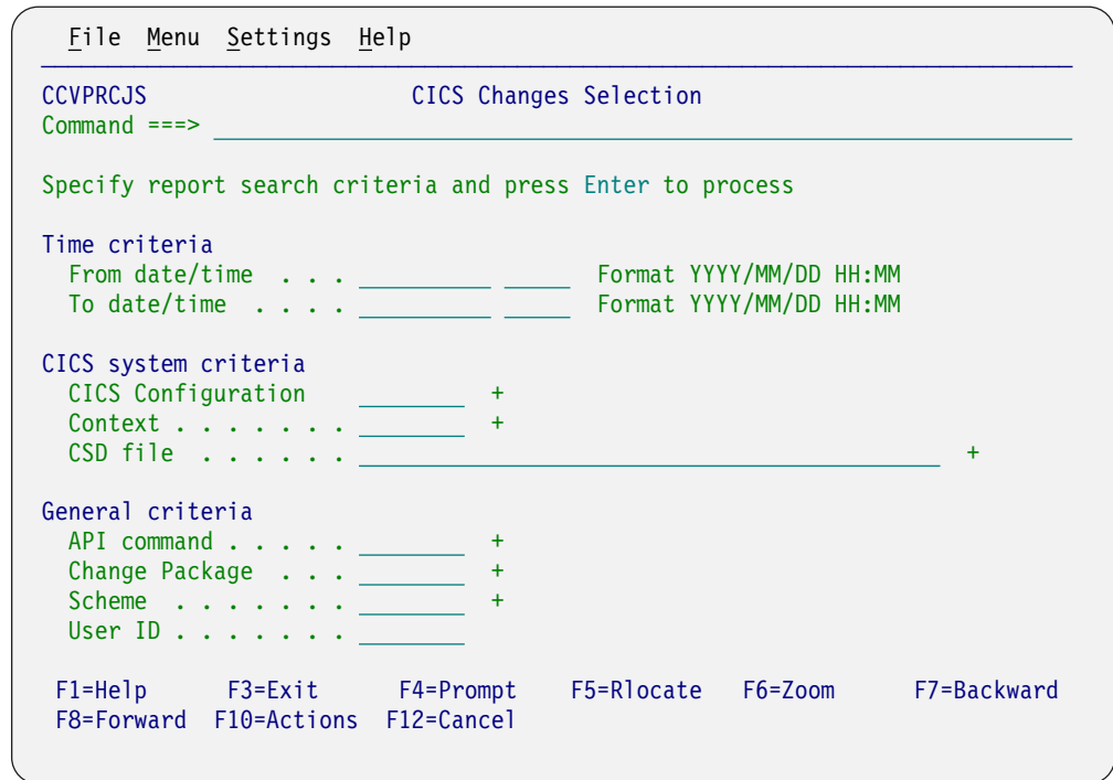
Figure 88. ISPF panel: CICS changes selection
