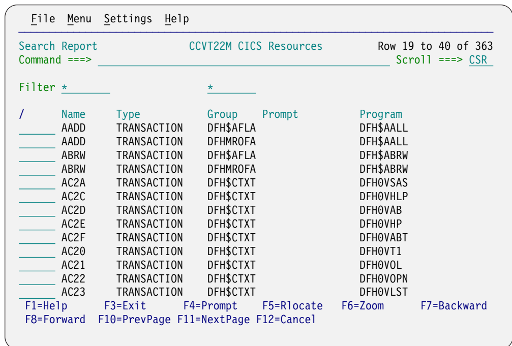
Figure 87. ISPF panel: report of transactions that use programs whose names match the pattern DFH*
