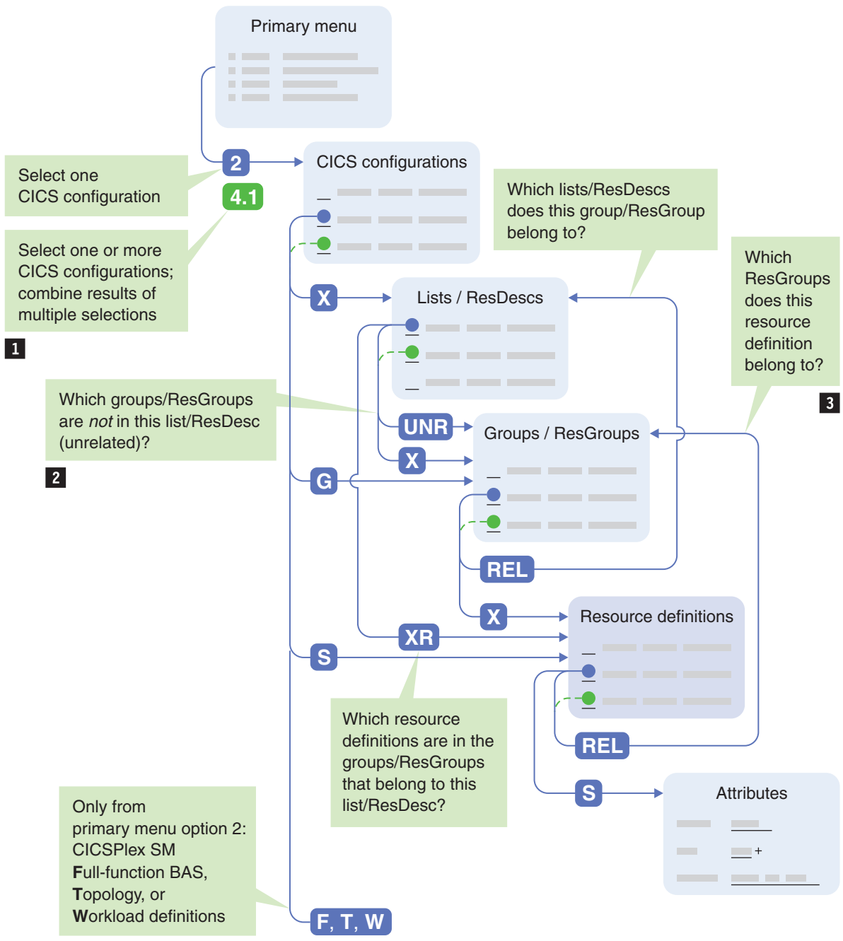
Figure 78. How to explore a CICS configuration hierarchy (or go directly to a list of resource definitions)
